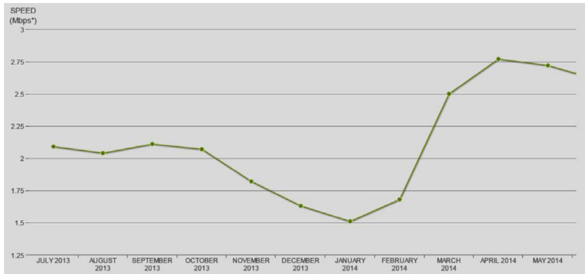
Figure 2: Performance of Netflix traffic to its customers over Comcast's network (July 2013 to May 2014)
